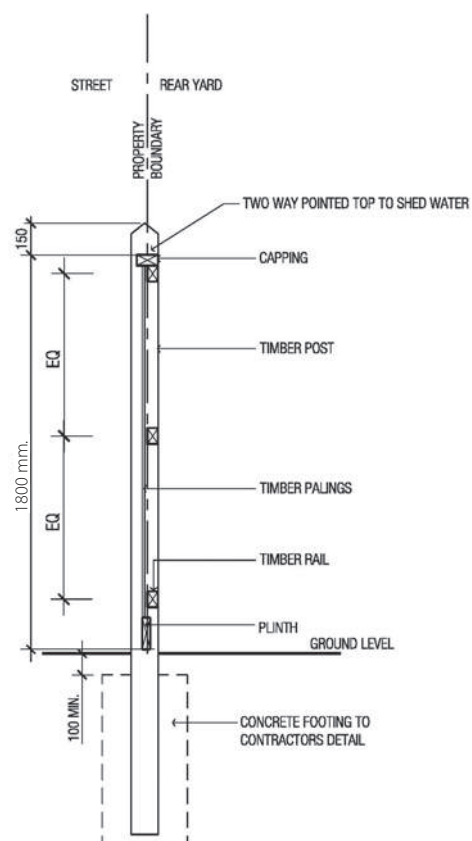
Character Precinct 3 - Secondary Frontage Lot Boundary Fence Detail
