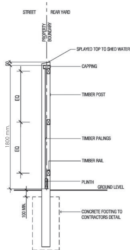
Character Precinct 1 - Secondary Frontage Lot Boundary Fence Detail
