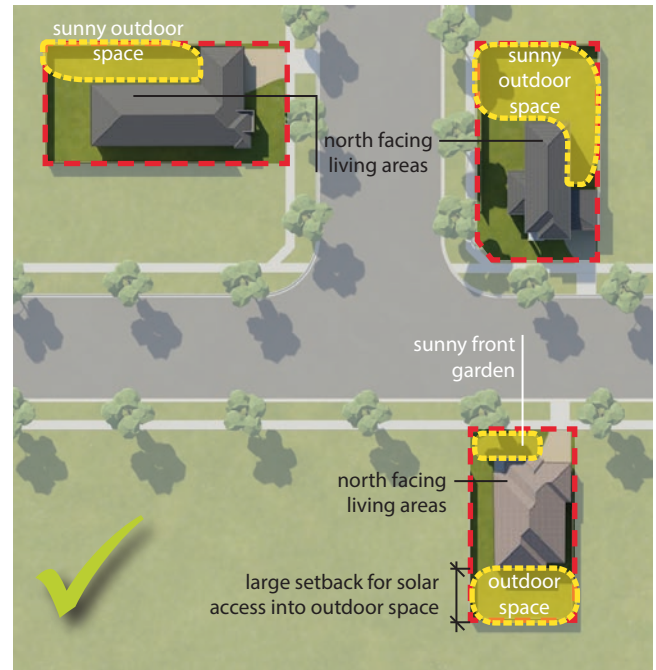
Diagram 18 - Site Layout and Orientation
